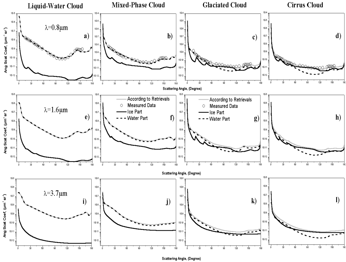
Figure 2. Extrapolation and projection of the angular scattering coefficients for the four types of cloud at three different wavelengths.
