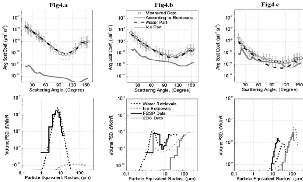
Figure 4. Inversion of the averaged scattering phase functions for three types of cloud :
