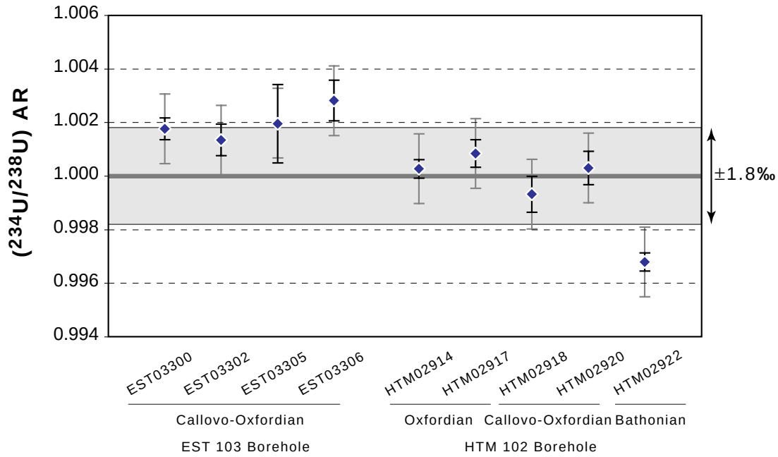
Figure IV. 2.: (^{234}\text{U}/^{238}\text{U}) activity ratio measurements on pristine samples from Bathonian and Oxfordian limestone and Callovo-Oxfordian argillite formations. Core samples are from the ANDRA HTM 102 and EST 103 boreholes. (^{234}\text{U}/^{238}\text{U}) activity ratios are calculated using the ^{234}\text{U}/^{238}\text{U} atomic ratio determined by Cheng et al. [28] for secular equilibrium material ( ^{234}\text{U}/^{238}\text{U} = 54,887.10^{-6} ). Reported error bars indicate either 2\sigma internal precision (black) or 2\sigma external reproducibility (grey).
