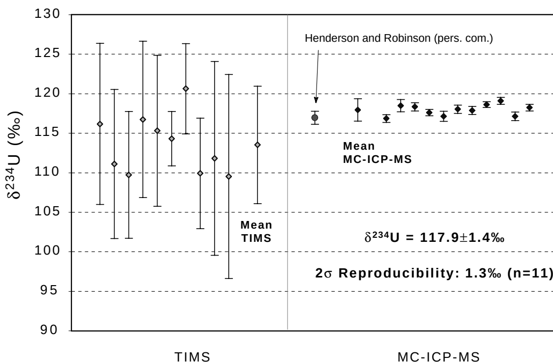
Figure I.6.: External reproducibility of the 234 U/ 238 U ratio (expressed as \delta^{234}\text{U} values) determined by replicate analyses of a coral sample (Barbados). Data are listed in Table 4. MC-ICP-MS results are compared with TIMS measurements also obtained at GEOTOP on a VG Sector TM mass spectrometer equipped with a 10 cm electrostatic analyzer and a pulse-counting Daly detector. Also reported is the analysis performed by Henderson and Robinson (pers. com.) on a Nu TM MC-ICP-MS at Oxford University (filled circle). All \delta^{234}\text{U} values are calculated using the half-life values determined by Cheng et al. (2000). Error bars represent 2 \sigma analytical precision. The MC-ICP-MS total external reproducibility is estimated to be \pm 1.3\text{‰} (2 \sigma , n=11).
