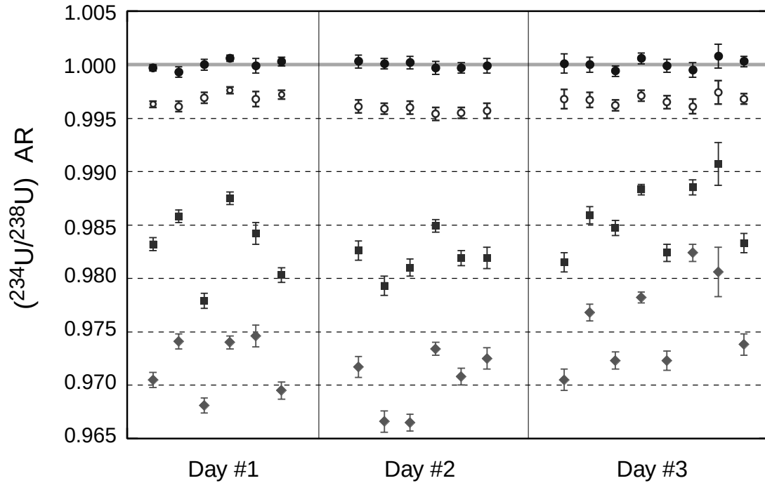
Figure I.1.: Repeated analyses of the (^{234}\text{U}/^{238}\text{U}) activity ratio of the HU-1 uraninite conducted on the Micromass IsoProbe TM MC-ICP-MS instrument over a 3-day analytical run. Results obtained using a tail correction based either on linear (filled diamonds) or exponential (filled squares) interpolation of half-mass zeroes are compared with results obtained using the tail correction method we developed (circles). The latter approach is based on the actual, precise quantification of tail contributions underneath each peak due to adjacent ion beams, as assessed by tail shape measurements on mono-isotopic ion beams. Blank circles refer to the correction which is done when the measured tail shape only is used; filled circles refer to results obtained by this same model using the tail shape corrected according to the \theta coefficient (see full explications in the text).
