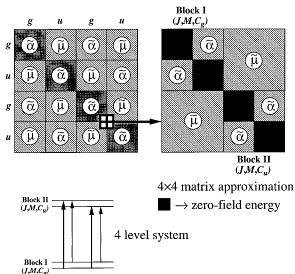
FIG. 3. The 4 × 4 matrix approximation for static Stark effect.
