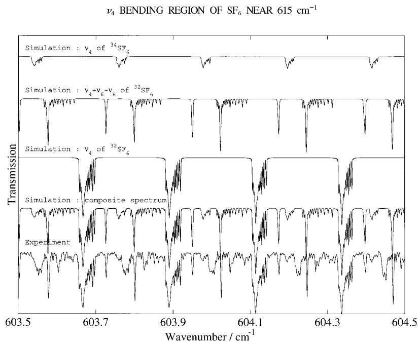
FIG. 4. Experimental and simulated spectra in the P -branch region.
