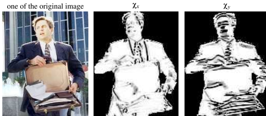
Fig. 2.38: Sample \chi_x and \chi_y functions
