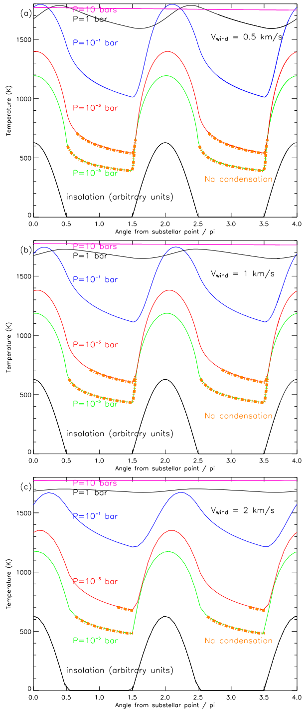
Fig. 5. Temperature at selected levels as a function of longitude for an equatorial wind velocity of (a) 0.5 km sec -1 (b) 1 km sec -1 and (c) 2 km sec -1 . The incoming insolation is shown in arbitrary units. Note the shift of the maximum of temperature with respect to the maximum of insolation (at the substellar point) as depth (and so the radiative timescale) increases. Below the 10-bar level, the temperature field is essentially uniform.
