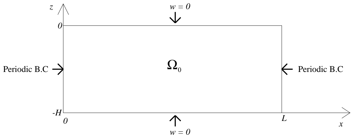
Figure 6.1: Domain \Omega_0
