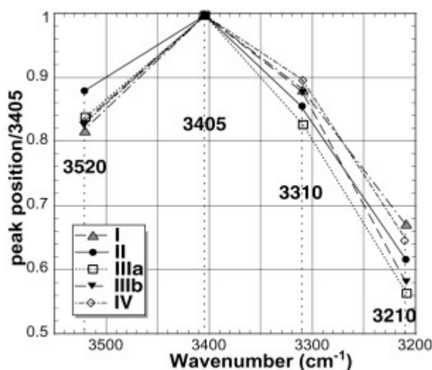
Figure 10 : Peak intensities of 3520, 3310 and 3210 cm -1 components relative to 3405 cm -1 in fluid inclusion IR spectra at room temperature.
