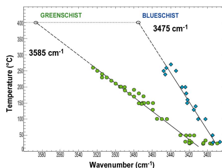
Fig. 4: Evolution of peak position of O-H IR spectra with temperature for fluid inclusions trapped in blueschist and greenschist facies conditions, with extrapolation to 400°C.
