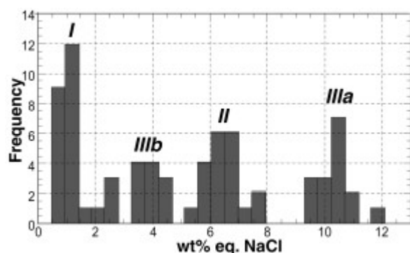
Figure 3 : Frequency histograms of salinities encountered in H 2 O-NaCl fluid-inclusions. a) Peak frequency in FI I (sample I) is centered on 1 %wt eq. NaCl. b) Sample II fluid-inclusion salinities are centered on 6.4 %wt eq. NaCl (FI II). c) Salinity in FI IIIa H 2 O-NaCl inclusions (sample III) range between 10 and 10.5 %wt eq. NaCl.
