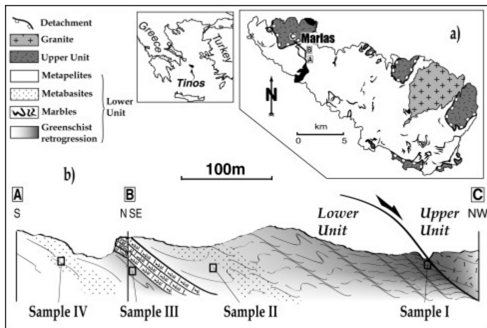
Figure 1 : a) Simplified geological map of Tinos Island (after Mélidonis, 1980), with cross-section locations A, B and C. b) Sample locations within a cross-section of the uppermost Lower Unit underlying the major detachment.
