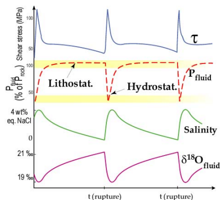
Figure 3: Seismic pumping model in the ductile regime, compared with fluid inclusion and isotope data.
