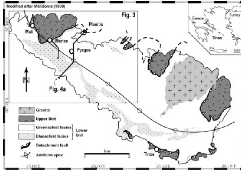
Figure 1 : Simplified geological map of Tinos Island (After Mélidonis, 1980).
