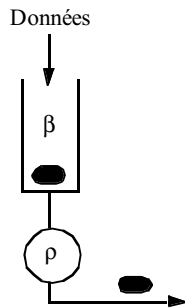
Figure 8: Leaky Bucket
