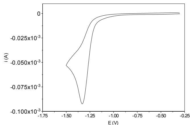
Figure III-5. Cyclic voltammogram of 2,6-lutidinium tetrafluoroborate (0.4 M, 0.2 M [\text{NBu}_4][\text{BF}_4] in acetonitrile, 0.1 \text{ V}\cdot\text{s}^{-1} ).
