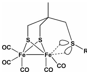
Scheme II-15. Postulated transition state for the inversion of the two lone pair electrons of the thioether ligand.
