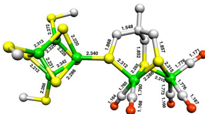
Figure IV-11. Structure of [Fe 4 S 4 (SCH 3 ) 3 {Fe 2 (CO) 5 (CH 3 C(CH 2 S) 3 )] 2- , derived from DFT calculations (bond lengths in Å).
