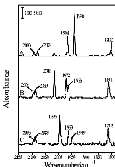
Figure I-3. FTIR spectra of DdH: (A) H_{ox-active} ; (B) H_{ox-active} -CO; (C) H_{ox-active} - 13 CO (taken from reference 29 ).
