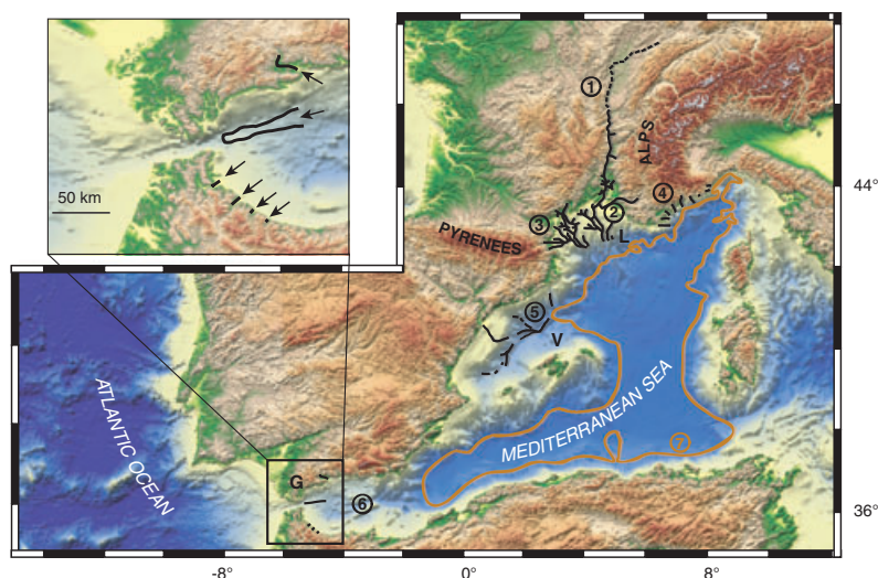
Fig. 1 Digital Elevation Model image of the western Mediterranean region (source: http://edcdaac.usgr.gov/gtopo30/gtopo30.asp ) showing the main Messinian rivers. 1, Rhone (after Clauzon, 1982; Clauzon et al. , 1995; Baumard, 2001); 2, Gulf of Lion shelf (after Guennoc et al. , 2000); 3, Languedoc (after Clauzon et al. , 1987; Ambert et al. , 1998); 4, Var and Ligure (after Clauzon, 1978); 5, Valence (after Field and Gardner, 1991); 6, Western Alboran Sea (after Morel, 1987; Campillo et al. , 1992; Schoorl and Veldkamp, 2003); 7, Limit of the Messinian evaporites (after Rouchy and Saint Martin, 1992). L, Gulf of Lions; V, Valence trough; G, Gibraltar strait.
