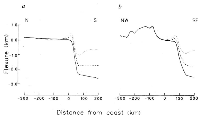
Flexural effects combined with present topography, giving a regionally compensated palaeotopography profile from 200 km offshore to 300 km onshore, assuming D = 10^{23} N m. Solid line, present profile; broken line, latest Messinian palaeotopography, calculated by removal of water load; dotted line, early Messinian palaeotopography, calculated by removing both water and salt loads (density 2,200 \text{ kg m}^{-3} ). a, N7E through Rhone Valley, slight uphill gradient. b, N38W through Cape d'Agde, moderate uphill gradient.
