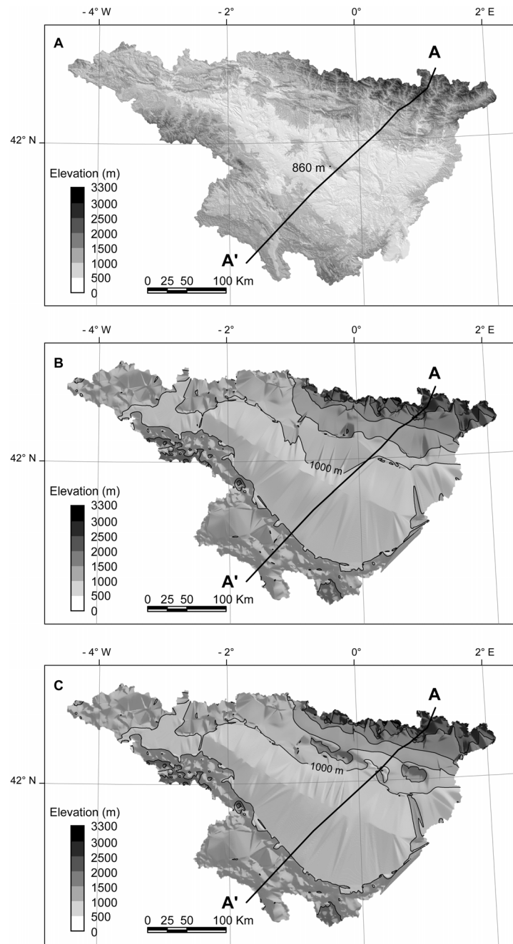
Figure 3: Miocene paleotopography.
