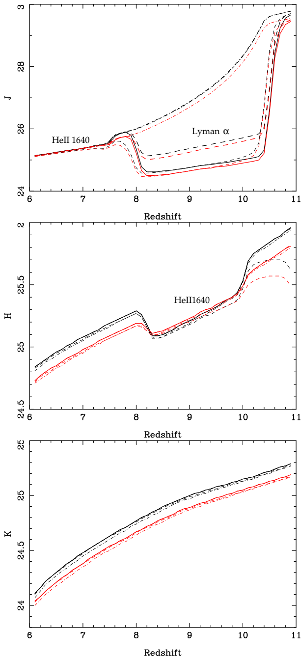
Fig. 4. From top to bottom, J , H and K s magnitudes as a function of redshift for a top-heavy IMF, for a fiducial stellar halo of 10^7 M_{\odot} . The values corresponding to a normal Salpeter IMF are about 2 magnitudes fainter over all the redshift interval. Black and red lines correspond respectively to burst ages 10^4 and 10^6 yrs. Various models for Pop III objects are presented, for different fractions of the Lyman- \alpha emission entering the integration aperture: 0 % (thick dot-dashed line), 50 % (thick dashed line), and 100 % (thick solid line). Thin dot-dashed lines correspond to a self-consistent extended Lyman- \alpha halo emission (Loeb & Rybicki 1999), whereas thin dashed lines display the same model with 100 % of Lyman- \alpha emission entering the integration aperture.
