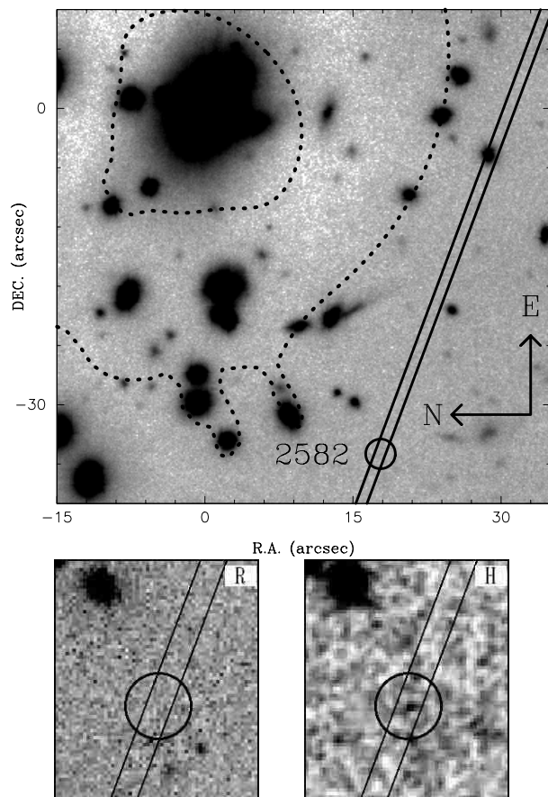
Fig. 1. Composite JHKs ISAAC image of the cluster Abell 1835 (top), showing the location of object #2582 (circle) and the slit configuration used for spectroscopy with ISAAC. Superposed are the theoretical critical lines at z = 1.6755 . On the bottom, close-ups images in the R -band ( F702W ) HST/WFPC2 (left) and the H -band ISAAC, smoothed with a \sigma = 1 pixel Gaussian (right).
