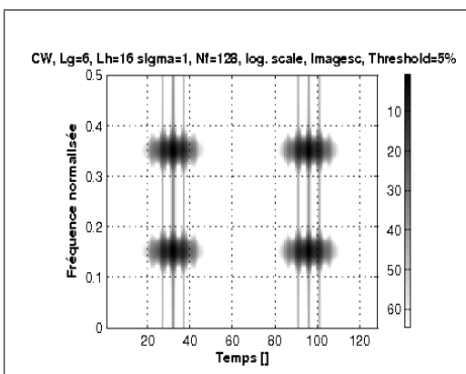
(e) Choi-Williams.
