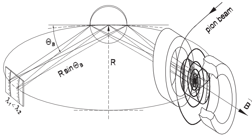
Figure 3.1 – The Johann-type crystal spectrometer set-up. X-rays with different energies are reflected by the crystal with different angles, therefore they form different lines in the position sensitive detector.
