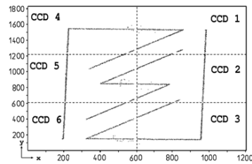
FIG. 11: Pattern produced by sulphur K\alpha radiation excited by means of an X-ray tube.
