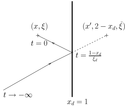
Figure 4.3: Total reflection
