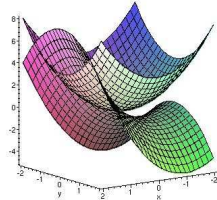
Figure 4.2: Two quadrics whose intersection curve I projects onto the parabola C : x = y^2 . Interpolation points located on I do not uniquely define an interpolating height function.
