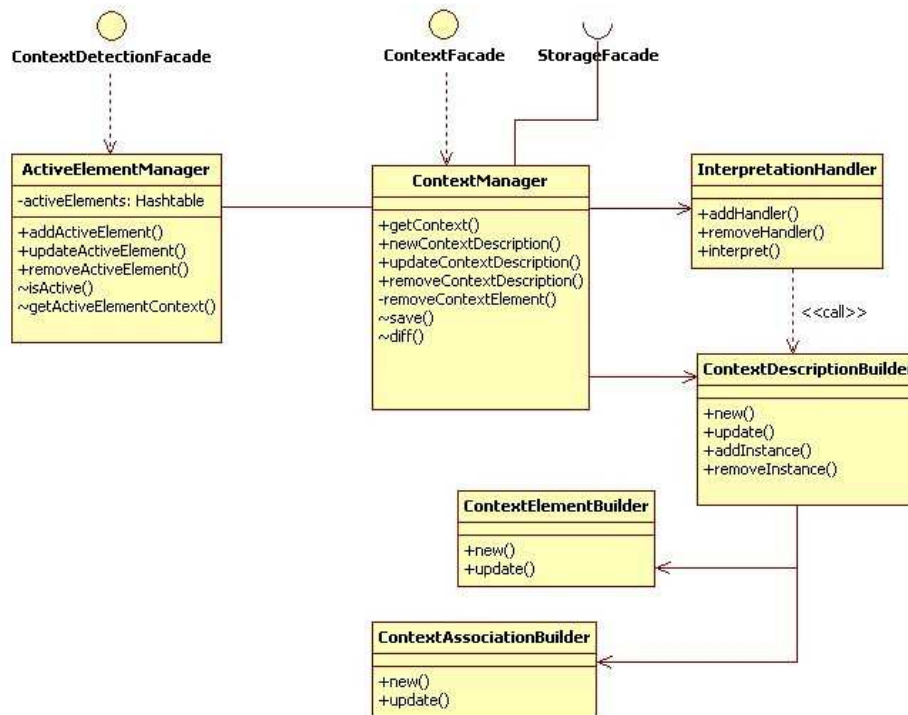
Figure 77. Classes qui composent la gestion des instances.
