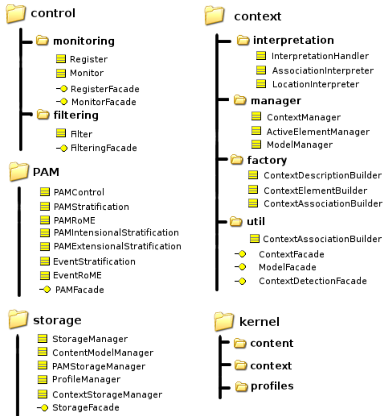
Figure 84. Paquetages Java du canevas BW-M.
