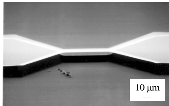
b) Pont 10 \mu\text{m} \times 50 \mu\text{m}
