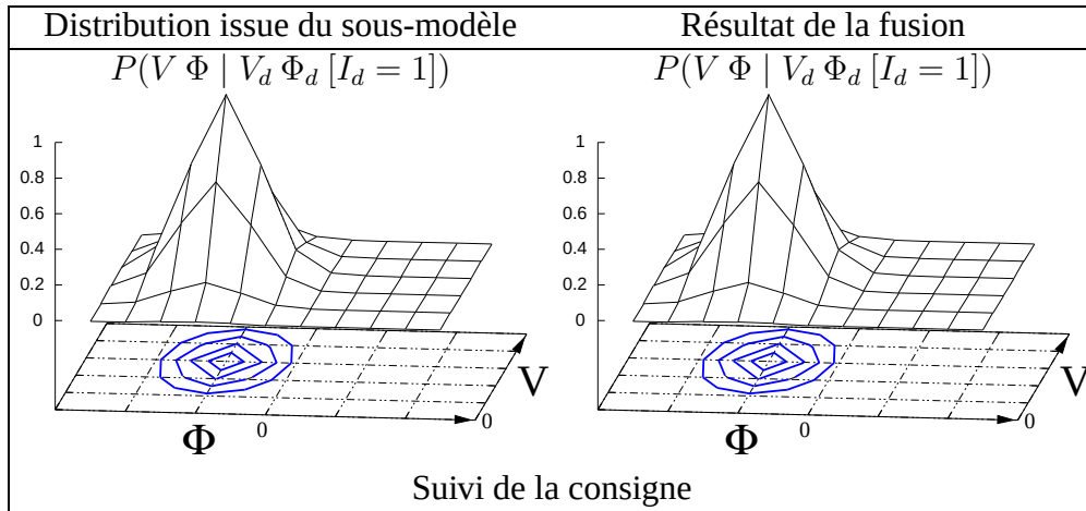
FIG. 6.14: Calcul progressif de P((V, \Phi) \mid (V_d, \Phi_d) D_1 \dots D_8 [I_i = 1]_{i=1 \dots 8} [I_d = 1]) , étape 1.
