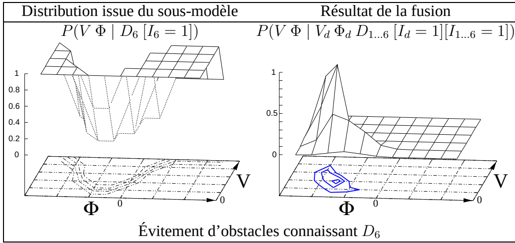
FIG. 6.17: Calcul progressif de P((V, \Phi) \mid (V_d, \Phi_d) D_1 \dots D_8 [I_i = 1]_{i=1\dots 8} [I_d = 1]) , étape 4.
