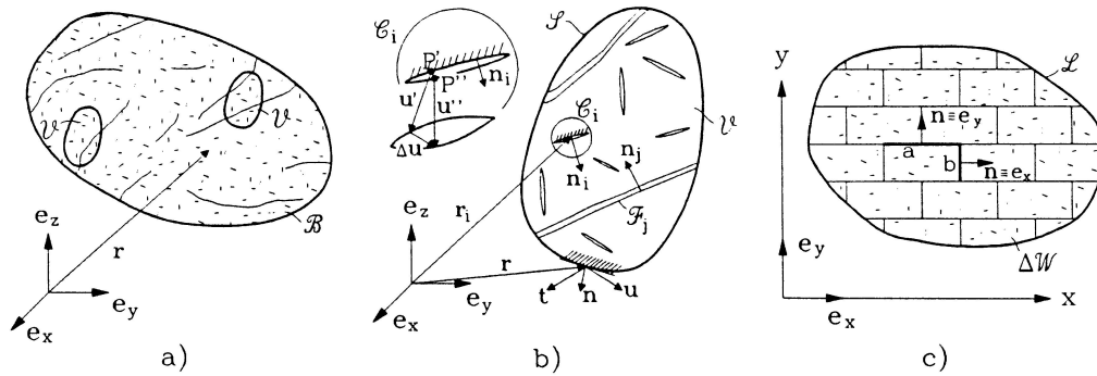
FIG. 1. (a) Small portions \mathcal{V} of a body \mathcal{B} containing microcracks and parts of large flaws ; (b) displacement jumps at microcracks and flaws ; (c) portion \Delta \mathcal{W} of a masonry wall.
