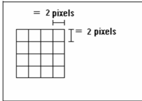
Figure 42 : Matrice M2
