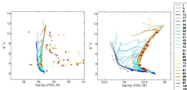
FIG. 3 – Uncalibrated \theta - S profiles for float n^{\circ} 1900042 (solid lines) compared with the estimated salinity correction from the objective analysis along theta levels for each profile (circles). Left panel : correction based on WOD2001 historical database ; right panel : SODB2005 historical database. The colours show the time evolution from cycle 1 (blue) to cycle 108 (red) three years later. The float starts south of the SAF (cold fresh profiles) and moves north of the front (warm, salty profiles) passing through the frontal region with strong interleaving.
