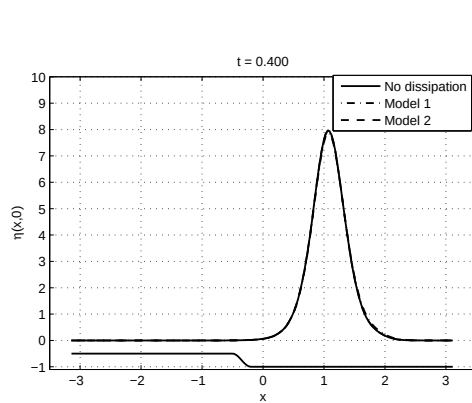
Figure 2.11: Free-surface snapshot before the interaction with the step: (left) the curves corresponding to the three models are almost superimposed; (right) difference between model II and model I.
