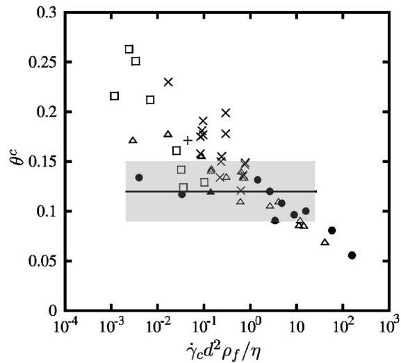
FIG. 5. Critical Shields number \theta^c vs \gamma_c d^2 \rho_f / \eta : experimental data of Charru et al. (Ref. 8) (▲), of Loiseleux et al. (Ref. 9) (●), of White (Ref. 6) cited by Loiseleux et al. (Ref. 9) (+), of White (Ref. 10) cited by Mantz (Ref. 11) (□), of Mantz (Ref. 11) (×), and of Yalin and Karahan (Ref. 7) (△). The solid line represents our result with the gray rectangle indicating the error range.
