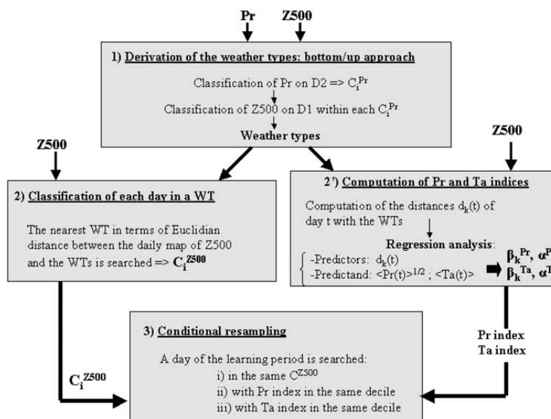
Figure 2. Flowchart presenting the main step of the downscaling algorithm “weather typing 1” for a season. Pr is precipitation, Ta is temperature and Z500 is 500 hPa geopotential height. WT is weather type. C_i^{Pr} is the ensemble of the days that belong to the precipitation cluster i . C_i^{Z500} is the ensemble of the days that belong to the weather type i . The \beta_k are the regression coefficients and \alpha the constant of the regression equations (index Ta for temperature and index Pr for precipitation).
