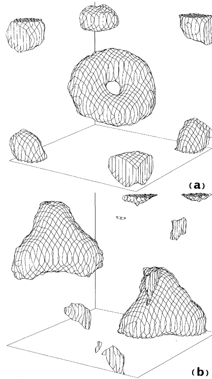
FIG. 2. Atomic position distributions in the cell -\lambda/2 < x, y, z < \lambda/2 , for a j_g = 2 \rightarrow j_e = 3 transition, with h|\delta|s/2E_{Rec} = 30 and \delta = -5\Gamma . The probability of finding the atom within the surfaces of constant density shown is 1/4 . The corresponding enclosed volume is 6% for (a) (vanishing phases) and 8% for (b) [phases (0, \pi/3, 2\pi/3) ].
