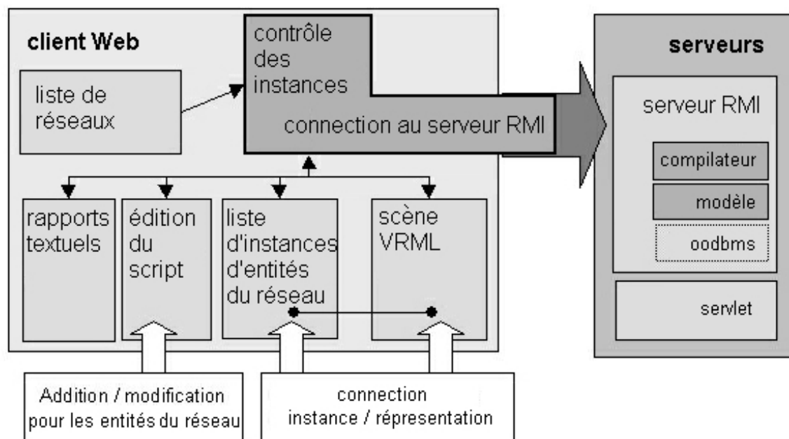
Figure 159 Architecture Client / Serveur de l'application HUBLOT
