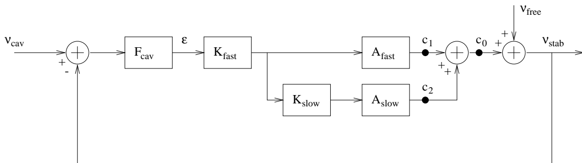
Figure 2: Servo loops related to the previous frequency stabilisation system
