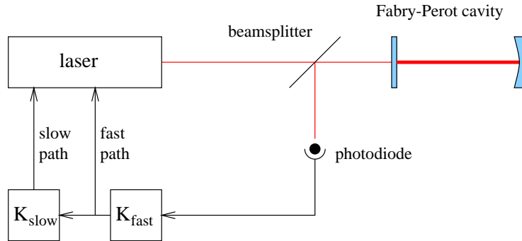
Figure 1: Laser stabilized in frequency on a Fabry-Perot cavity
