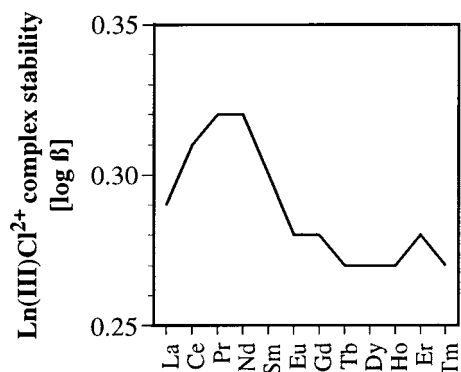
Fig. 9. Plot of the complex stability constants of \text{Ln}(\text{III})\text{Cl}^{2+} lanthanide complexes. The constants are infinite dilution values from Millero (1992). The values for Yb and Lu are below 0.25 and not shown to limit the scale of the figure (Yb = 0.16; Lu = -0.03).
