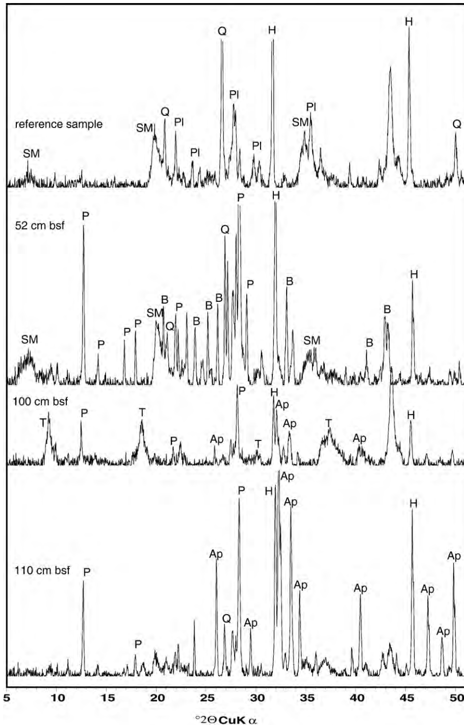
Fig. 4. XRD patterns of the reference sediment and three GC50 samples showing the mineralogical changes with depth. Peak labels: B = barite, Ap = apatite, H = halite, P = phillipsite, Pl = plagioclase, Q = quartz, SM = smectite, T = todorokite.
