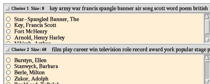
Figure 23 - Grouper [Zamir, 1999]
