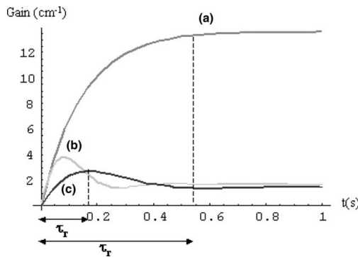
Fig. 2. Temporal evolution of local gain at different intensities at T = 297 K ( e_n^h = 16.31 \text{ s}^{-1} calculated from Eq. (17)), A = 5 \mu\text{m} , E_0 = 10 \text{ kV/cm} , crystal thickness L = 12 \text{ mm} : (a) I_0 = 25.5 \text{ mW/cm}^2 \sim I_{res} , (b) I_0 = 15 \text{ mW/cm}^2 and (c) I_0 = 50 \text{ mW/cm}^2 . \tau_r : characteristic time constant of amplification.
