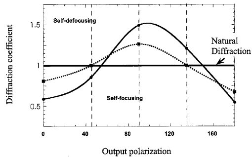
FIG. 8. Averaged diffraction coefficient measured for a 3.17 \text{ mm} long BTO crystal for an input beam waist of 30 \mu\text{m} , a fluence of 5 \text{ mJ/cm}^2 , and applied fields of 6.25 \text{ kV/cm} (solid line) and 3.75 \text{ kV/cm} (dotted line) as a function of the output polarization.
