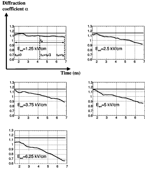
FIG. 3. Measured time evolution of the diffraction coefficient \alpha(t) during a pulse duration \tau_p taken in the direction parallel to the applied electric field, for w_e = 20 \mu\text{m} , d_e = 5 \text{ mJ/cm}^2 , P_s = 0^\circ and for different applied fields: (a) 1.25 kV/cm, (b) 2.5 kV/cm, (c) 3.75 kV/cm, (d) 5 kV/cm, and (e) 6.25 kV/cm.
