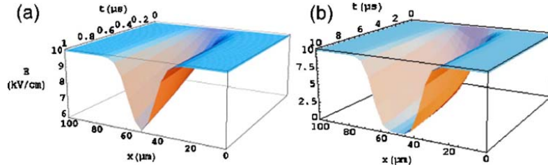
FIG. 4. (Color online) Space-charge field buildup for a duration of 1 \mu\text{s} (a) and for a duration of 10 \mu\text{s} (b) as a function of time and space.
