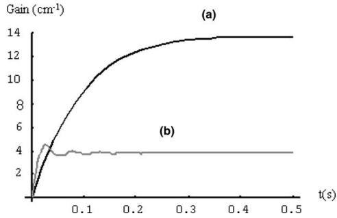
Fig. 4. Local (a) and average gain (b) versus time, I_0 = 25.5 \text{ mW/cm}^2 , \epsilon_n^{\text{th}} = 16.31 \text{ s}^{-1} , \Lambda = 5 \mu\text{m} and E_0 = 10 \text{ kV/cm} .
