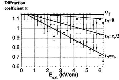
FIG. 4. Experimental diffraction coefficient \alpha vs the external applied electric field for w_e = 20 \mu\text{m} , d_e = 5 \text{ mJ/cm}^2 , and P_s = 0^\circ at different times during the pulse: t_N = 0 , t_N = \tau_p/2 and t_N = \tau_p .
