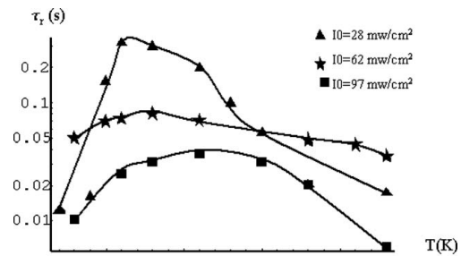
Fig. 8. The \tau_r versus temperature at different intensities.
