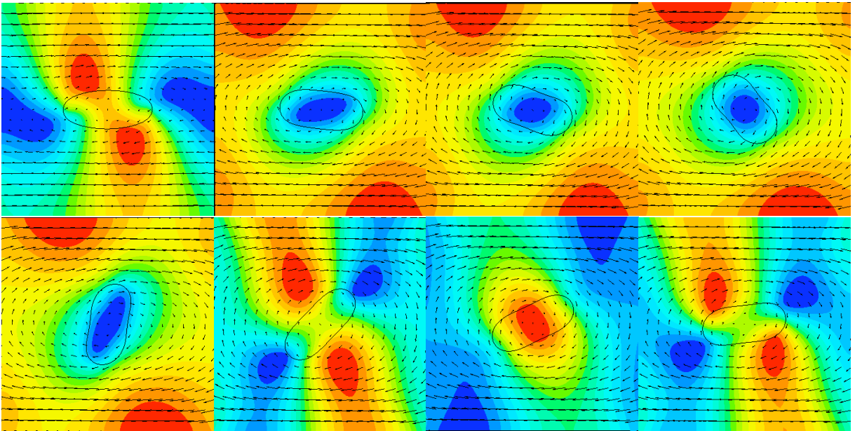
FIGURE 14: Tumbling motion of vesicle in a shear flow. Viscosity contrast: 4. Reynolds: 4.10^{-4} . Colors stand for iso-pressure lines.
