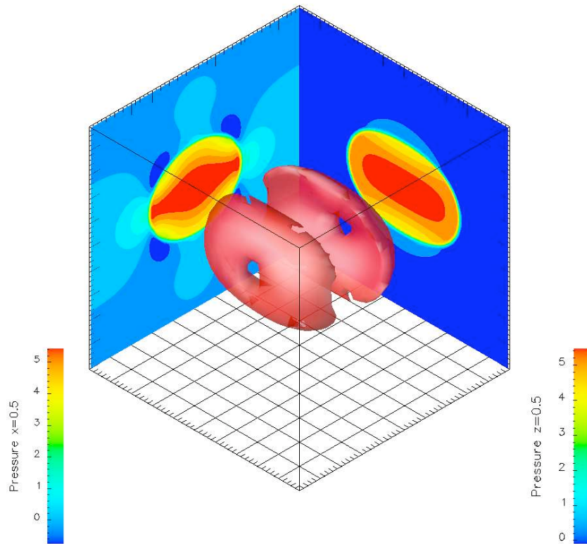
FIGURE 1: Iso-vorticity surface in the relaxation of an elastic immersed membrane
