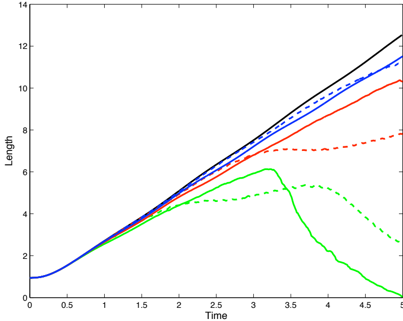
FIGURE 9: Comparison between reinitialization (dashed lines) and renormalization (continuous lines) for N = 64, 128, 256 , in a test where an interface is stretched by a rotating velocity field. Top curve is a high resolution front tracking solution.
