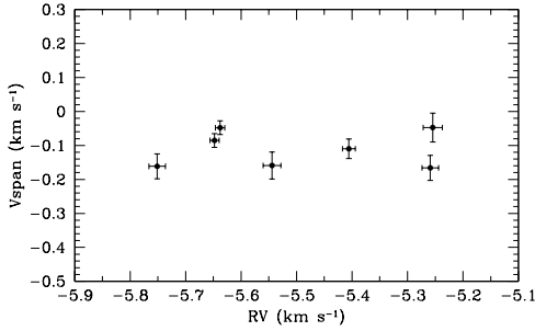
Figure 4. Analysis of line-bisectors in WASP-3 shows the bisector velocity ( vspan ) does not correlate with stellar radial-velocity. This demonstrates that the cross-correlation function remains symmetric, and that the radial-velocity variations are not likely to be caused by line-of-site binarity or stellar activity.
