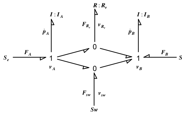
Fig. 5. Acausal bond graph representation of a two-body system with friction
