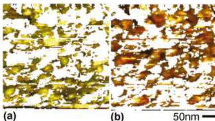
FIG. 3. (Color) (a) Map of Ag clusters determined by the ratio of photon intensity in the ranges 620–730 nm and 480–540 nm. (b) Map of remaining Cu clusters.
