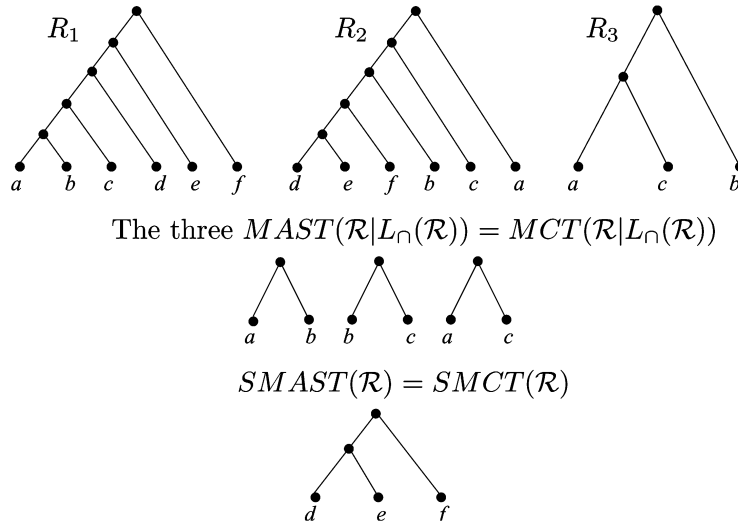
Fig. 6. A collection \mathcal{R} = \{R_1, R_2, R_3\} of rooted input trees for which the trees \text{MAST}(\mathcal{R}) and \text{MCT}(\mathcal{R}) can not be used as backbones of \text{SMCT}(\mathcal{R}) and \text{SMCT}(\mathcal{R}) .
