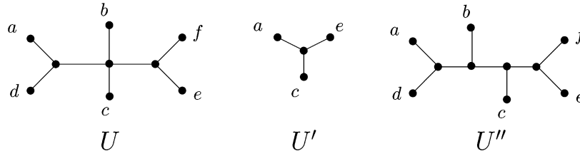
Fig. 1. Three unrooted trees. A tree U , a tree U' such that U' = U|_{\{a, c, e\}} and a tree U'' such that U'' \supseteq U .
