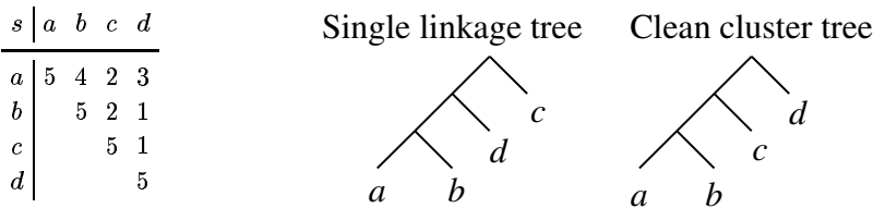
FIG. 1. A similarity function s on four points, its single linkage tree and clean cluster tree.
