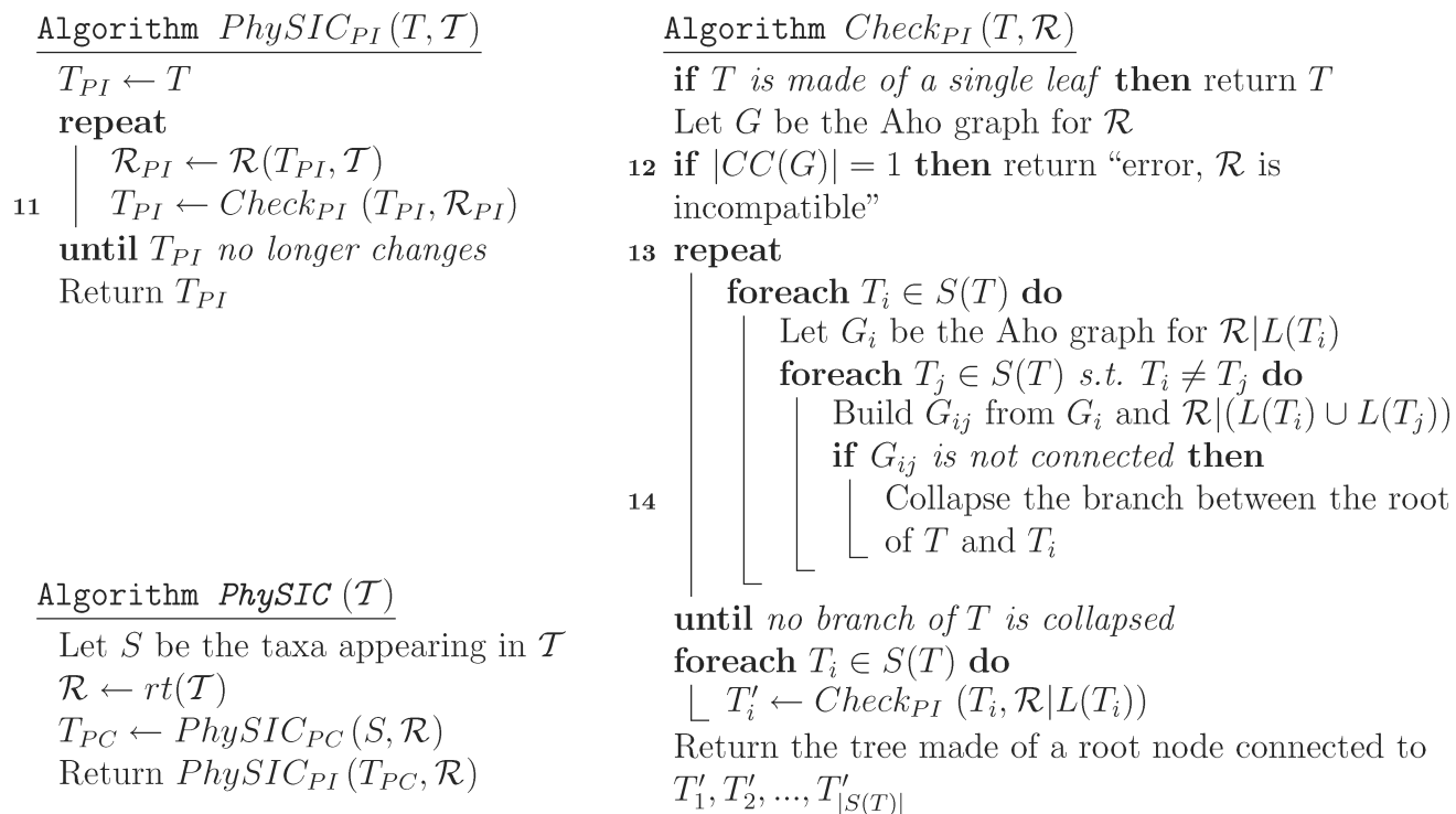
FIGURE 10. Details of the PhySIC algorithm and PhySIC PI and Check PI subroutines.
