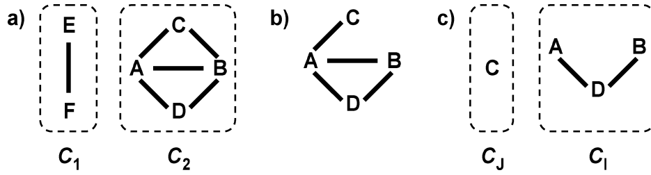
FIGURE 7. Examples of graphs. (a) The initial Aho graph G created from the triplets rt(T) of the collection T displayed in Figure 2. The two connected components of G are C_1 = \{E, F\} and C_2 = \{A, B, C, D\} . (b) The Aho graph obtained from \mathcal{R}|v(C_2) . This graph is connected, showing that the input trees conflict on the resolution of \{A, B, C, D\} and hence are incompatible. (c) The Aho graph obtained from \mathcal{R}|v(C_2) when removing the triplets \mathcal{R}_{dc} = \{AB|C, AC|B\} .
