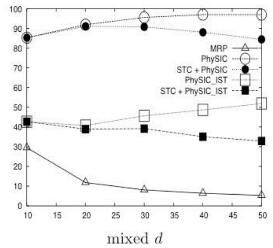
Figure B.3: Average percentage of type II error for various supertree methods, on input collections of 10 to 50 source trees depending on their overlap. Type II error is the percentage of edges in the correct tree (i.e. model tree) that are not contained in the inferred supertree.
