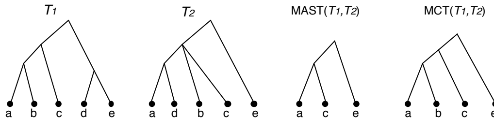
Figure 6.1: A collection \mathcal{T} = \{T_1, T_2\} of two incompatible trees, a maximum agreement subtree for \mathcal{T} and a maximum compatible tree for \mathcal{T} . Thanks to a less stringent definition, the MCT tree contains here more labels than the MAST tree.
