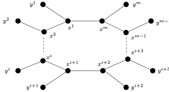
Fig. 9. The graph [G, L(G)] induced by the gadget G .
