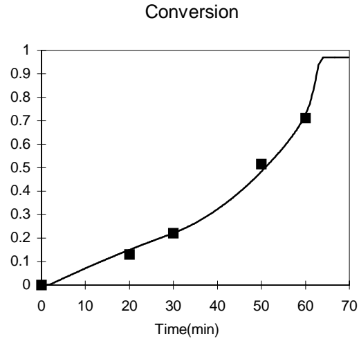
Figure 7.5: Overall conversion estimated (—) and gravimetric conversion (■).
