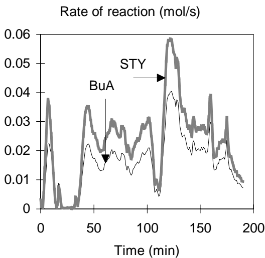
Figure 4.15c: Experiment 28/4/99. Estimated rate of the reaction of each monomer.
