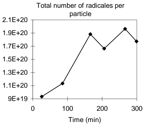
Figure 5.10g: N_P^T . Experiment 263.
