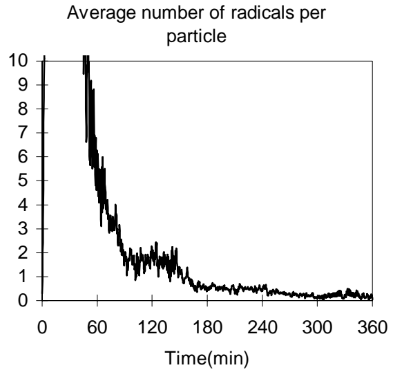
Figure 5.10h: \bar{n} .
