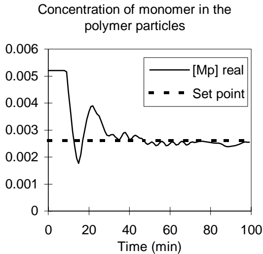
Figure 7.9c: Experiment C32. [M P ] (mol/cm 3 ).
