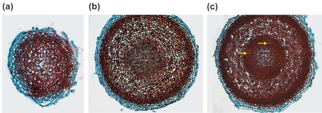
Fig. 4 Safranin-fast green staining of cross sections at different distances from the tip of the root cap: (a) 200; (b) 400; (c) 600 \mu\text{m} . In the sections, cellulose cell walls are stained green; cytoplasm and nuclei, red. Arrows, protophloem. Bar, 100 \mu\text{m} .
