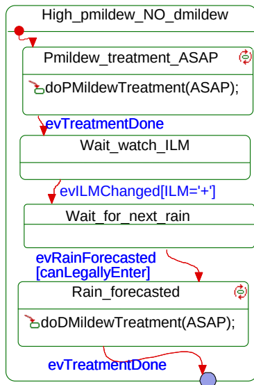
(b) High_pmildew_NO_dmildew substatechart
