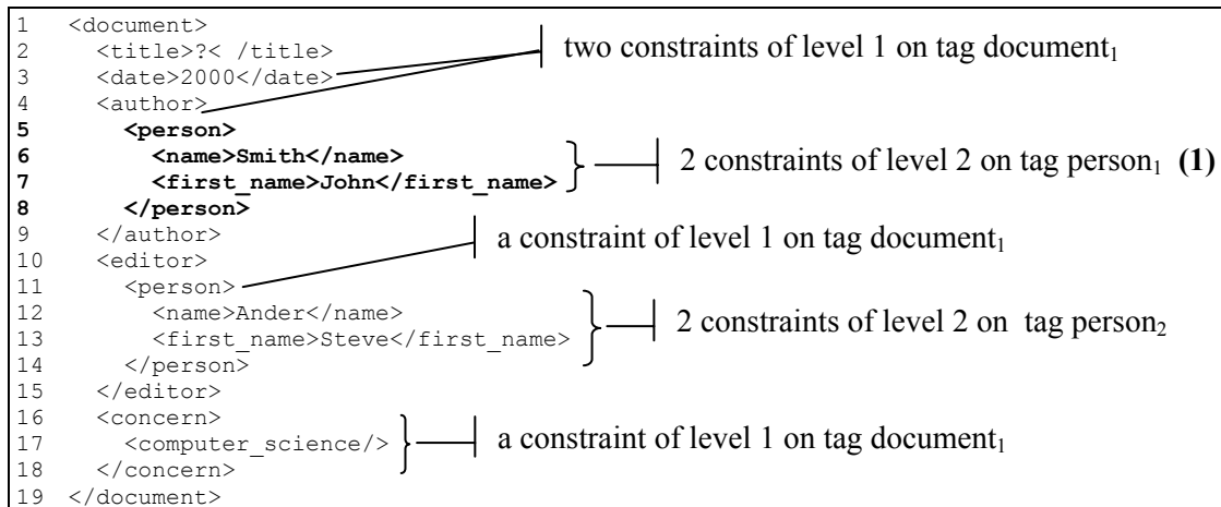
Figure 91 Anatomy of a sample query
