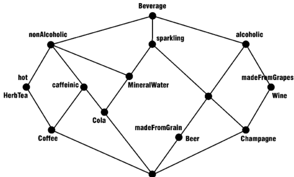
Figure 15 Revised lattice of beverage concepts [Sowa, 2000b]
