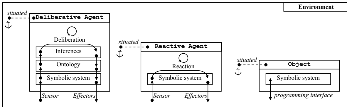
Figure 152 The three atomic entities of a complete distributed artificial paradigm
