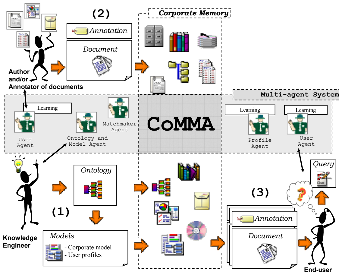
Figure 36 Overview of the approach
