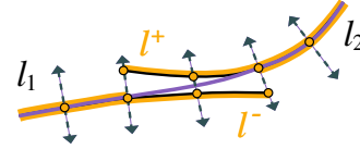
Figure 7: The hull (in orange) of a line l (in purple) representing a pair of lines (l_1, l_2) (in black) is defined by the farthest points of (l_1, l_2) along each normal of l (dashed line).
