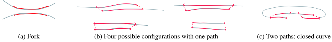
Figure 5: Possible configurations of a pair of \varepsilon -lines. Only (b) and (c) can form an \varepsilon -group.
