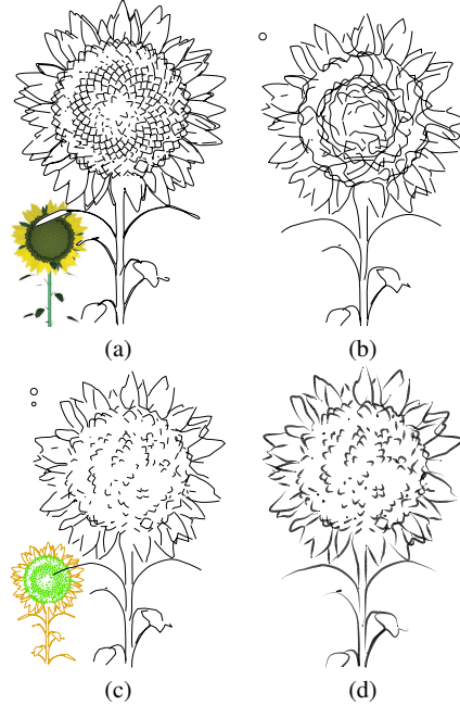
Figure 12: Simplification of a 3d rendering: (a) 3d model and its line rendering using silhouettes and suggestive contours (531 input lines) - (b) Simplification without any category (256 clusters) - (c) Using two categories (external and internal contours) each with a different scale and geometric strategy (294 clusters) - (d) Same result in a calligraphic style.
