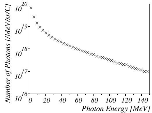
FIG. 3. Photon spectrum from Monte Carlo simulation averaged between 0^\circ and 1^\circ (with parameters T = 40 \text{ MeV} and \Theta_0 = 1^\circ for the electron beam converted in \gamma rays in a 2.5 mm-thick tantalum target followed by a 7.5 mm-thick aluminum foil).
