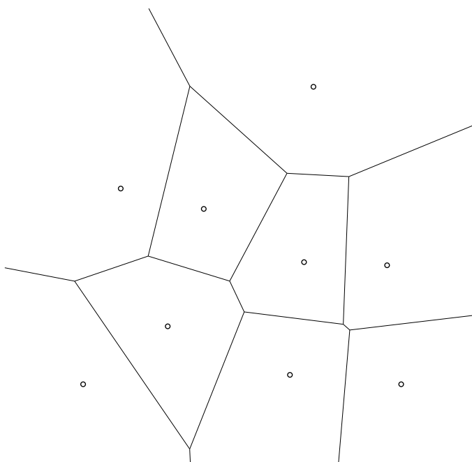
Figure 1: The Voronoi diagram of a set of 9 points.
