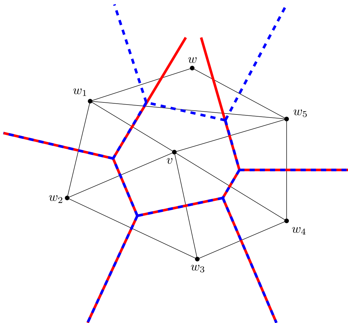
Figure 5.1: The local cell \text{Cell}_G(v) (solid lines) contains the power diagram cell (dashed lines) and contains another vertex w .
