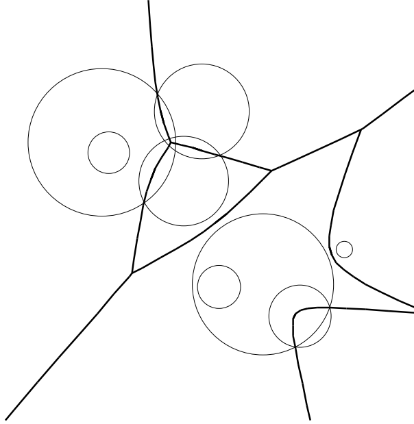
Figure 2.2: The Apollonius diagram of a set of circles. Compare with the power diagram of the same set of circles in Fig. 1.6.
