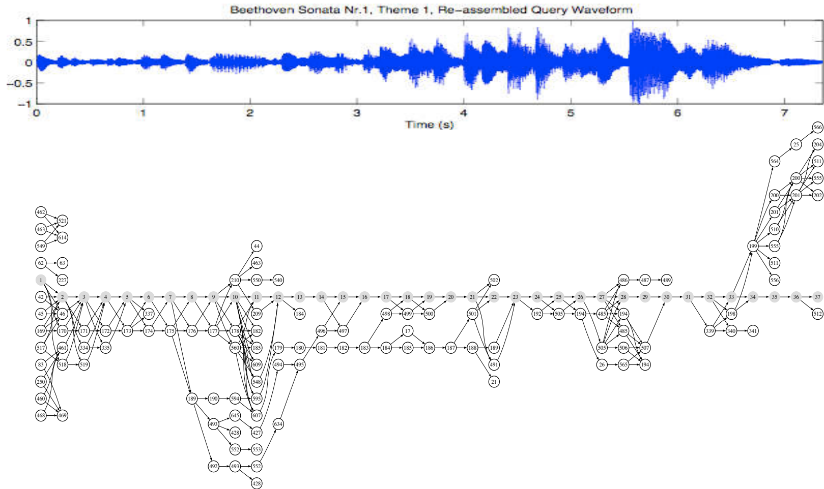
Figure 5.7: Model-Guidance sample results on Beethoven's Piano Sonata Nr.1-Mvt.1, using the first theme as audio query – Showing the reconstructed audio and the tree structure of the forward pass with best path highlighted in light-gray.
