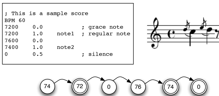
Figure 8.4: Antescofo 's single event score sample and state transition diagram
