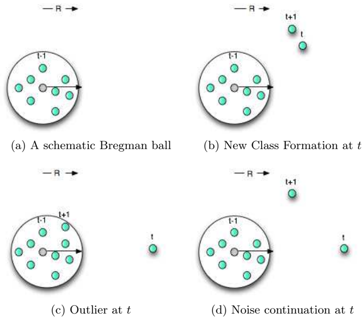
Figure 4.2: Schematic diagrams for incremental class formations using imaginary Bregman balls. Points correspond to continuous-time input vectors.
