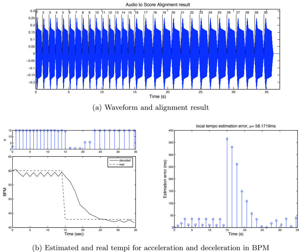
Figure 7.10: Tempo Decoding Evaluation using synthesized score and controlled tempo
