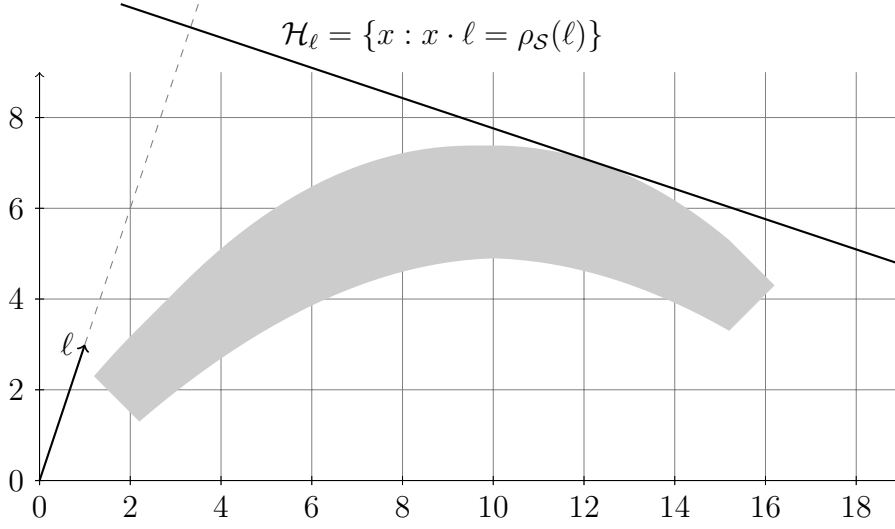
Figure 2.10: A set \mathcal{S} and its supporting hyperplane in direction \ell : \mathcal{H}_\ell .
