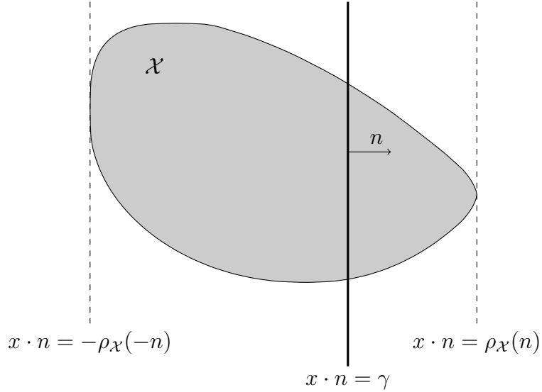
Figure 8.1: Checking emptiness of \mathcal{X} \cap \{x : x \cdot n = \gamma\} .
