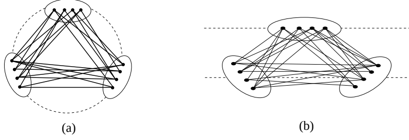
Figure 1.4: Tripartite request graphs used in Lemma 1.2: (a) in the ring for c = 1 ; (b) in the path for C = 2 .
