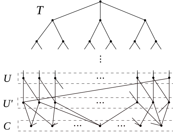
Figure 5.1: An example of the graph G built in the reduction of Theorem 5.9.
