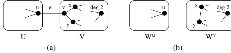
Figure 2.2: (a) A bridge e = \{u, v\} in an almost 3-regular graph G with components U and V of G - \{e\} . (b) Graphs smaller than G from which we obtain a partition into trails W^u and W^v .
