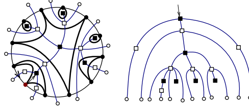
Figure 8.3: A non-crossing partition tree.
