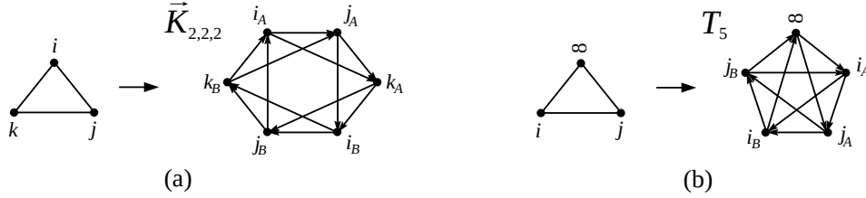
Figure 3.5: (a) Digraph \vec{K}_{2,2,2} obtained from K_3(i, j, k) , with i < j < k ; (b) digraph T_5 obtained from a K_3 of the form (\infty, i, j) .
