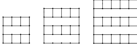
Figure 7.1: Connected subgraphs with maximum degree 3 on (4 \times 4) , (5 \times 5) , and (6 \times 6) -grids respectively, used in the proof of Lemma 7.3.
