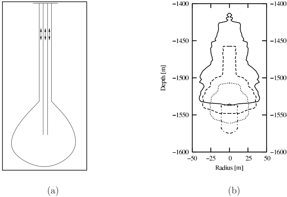
FIG. 1 – (a) Schematic of underground cavern in salt formation. (b) Average vertical sections obtained by sonar measurements at the end of four leaching steps.
