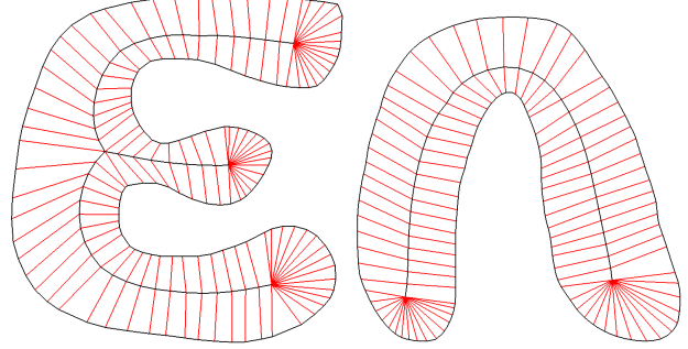
Fig. 1.6: New radial edges from our approach.
