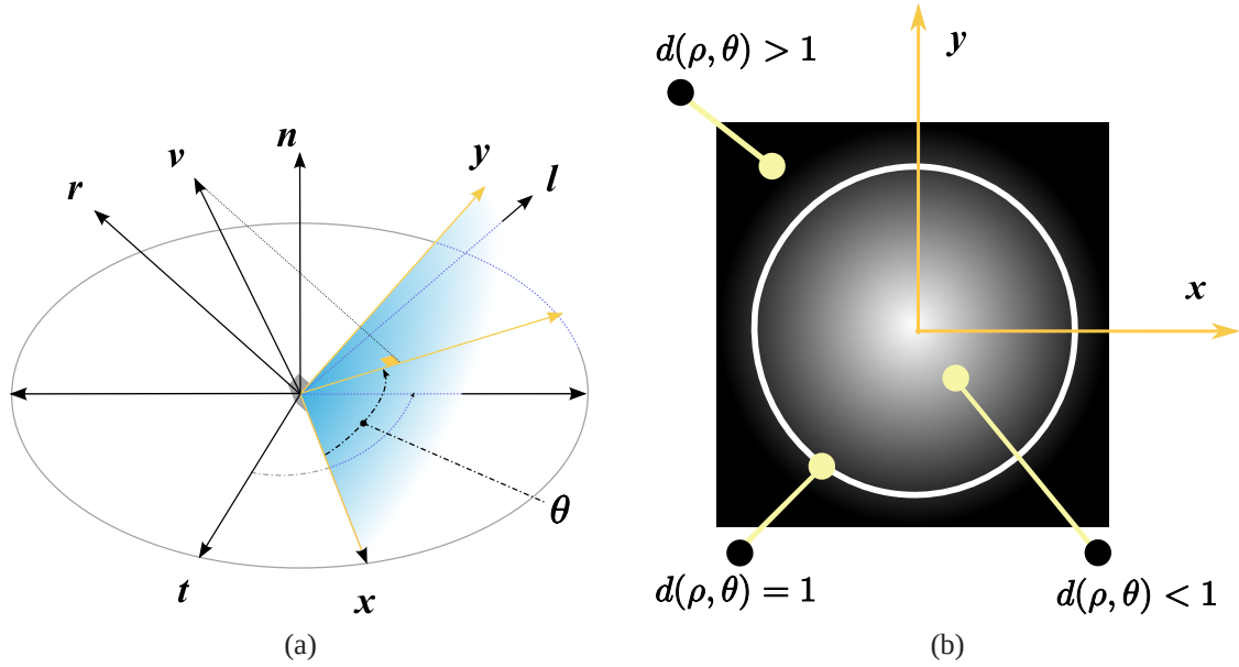
Fig. 2.5: (a) The x and y directions constitute the Sketching Plane local frame. They are computed according to the light mirror direction r and the geometry local tangent t . To compute the reflected intensity, we project the view direction v on the Sketching Plane. (b) The distance field d(\rho, \theta) defined by the polar curve parameterizes the Sketching Plane.
