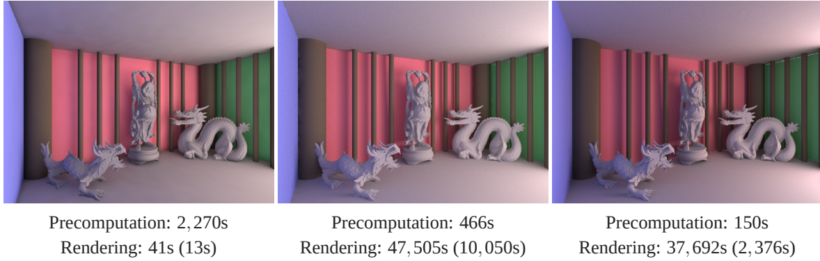
Fig. 3.12: Scene with mostly indirect illumination. (left) Our technique using directly a 30 \times 20 \times 92 uncompressed grid (11.4 MB) constructed with 80 M photons. (Center) Christensen’s method reference image with 3200 rays to sample the hemisphere and 5 M photons stored (124 MB). (right) Our technique using indirectly a 12 \times 8 \times 20 uncompressed grid (590 KB) with the same number of photons shot and the same number of rays to sample the hemisphere.
