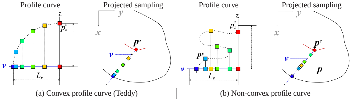
Fig. 1.1: Differences for surface elevation between Teddy and our approach: p_z^s is the silhouette elevation, v the direction of the radial edge and L_v its length. In Teddy (left), radial edges from skeleton to silhouette are sampled and the samples are elevated. In our approach (right), the profile-curve is sampled, and the position of these samples are adjusted for each radial edge, based on the local maximum elevation and edge length. The projection of the resulting 3D vertices on their corresponding radial edge is no more guaranteed to be ordered.
