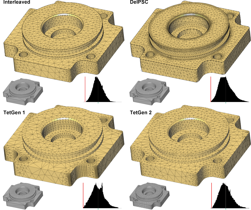
Figure 2.49: Cover rear. Top left: mesh obtained by interleaved refinement and optimization with l_{max} = 0.1 , \epsilon_{max} = 0.001 , \sigma_{max}^f = 1.5 , \sigma_{max}^t = 1.5 and the topology criterion activated. It contains 4,050 vertices and all dihedral angles are above 12.0 degrees. Top right: mesh generated by DelPSC, with the same parameters. It contains 15,157 vertices and all dihedral angles are above 0.1 degree. Bottom left: mesh generated by TetGen, with the same parameters and input. It contains 6,966 vertices and all dihedral angles are above 0.2 degree. Bottom right: mesh generated by TetGen, with the same parameters and the boundary of our optimized mesh taken as input. It contains 4,189 vertices and all dihedral angles are above 3.0 degrees.
