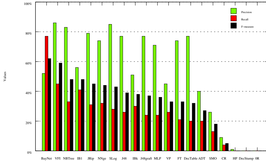
Figure 7.4: Average scores of each matcher over 200 scenarios
