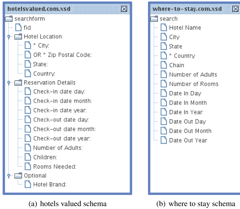
Figure 2.2: Two hotel booking schemas
