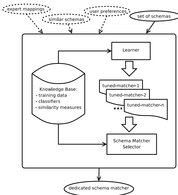
Figure 7.3: YAM architecture
