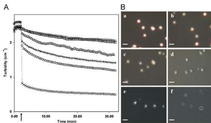
Fig. 4. (A) Destabilisation kinetic of LYS/apo \alpha -LA spherical particles by increasing the ionic strength ( I ) at 45 °C. The arrow shows the addition time of NaCl to the LYS/apo \alpha -LA mixtures. (B) Phase contrast micrographs of spherical particles taken 30 min after the addition of salt (scale bar: 5 \mu m). The final ionic strengths were: 39 mM (◇, a), 41 mM (□, b), 61 mM (△, c), 75 mM (+, d), 150 mM (○, e) and 250 mM (×, f). Spherical particles were pre-formed by mixing LYS (0.075 mM) and apo \alpha -LA (0.075 mM) in 30 mM Tris/HCl buffer (pH 7.5) containing 15 mM NaCl at 45 °C.
