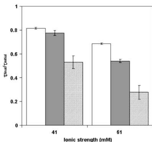
Fig. 6. Residual turbidity of LYS/apo \alpha -LA mixtures 30 min after their destabilisation by the addition of salts: NaCl (white), MgCl 2 (grey) and CaCl 2 (hatched). Spherical particles were pre-formed by mixing LYS (0.075 mM) and apo \alpha -LA (0.075 mM) in 30 mM Tris/HCl buffer (pH 7.5) containing 15 mM NaCl at 45 °C.
