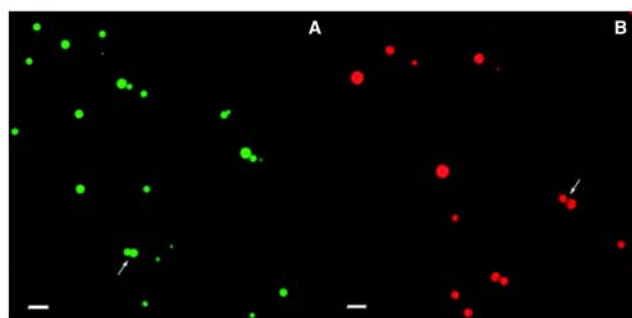
Fig. 1. Confocal scanning laser micrographs of microspheres prepared from apo \alpha -LA-FITC and unlabelled LYS (A) or unlabelled apo \alpha -LA and LYS-RBITC (B). Microspheres were obtained by mixing LYS (0.1 mM) with apo \alpha -LA (0.1 mM) in 30 mM Tris/HCl buffer, pH 7.5, containing 15 mM NaCl, and incubated for 30 min at 45 °C. Scale bars = 5 \mu m. Arrows indicate microspheres undergoing coalescence.
