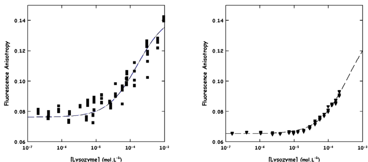
Figure 5. Specific binding curves of apo \alpha -LA – LYS (■) and holo \alpha -LA – LYS (▼) for an ionic strength of 124 mM at 45°C.
