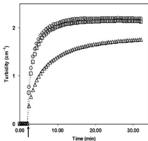
Fig. 3. Formation of LYS/apo \alpha -LA spherical particles in different buffers (pH 7.5) at 45 °C for a total ionic strength of 39 mM: (○) 30 mM Tris/HCl, 15 mM NaCl; (□) 10 mM phosphate, 15 mM NaCl; (△) 100 mM imidazole, 15 mM NaCl. Spherical particles were prepared by mixing LYS (0.075 mM) and apo \alpha -LA (0.075 mM) at 45 °C. The arrow shows the addition time of LYS to apo \alpha -LA solution.
