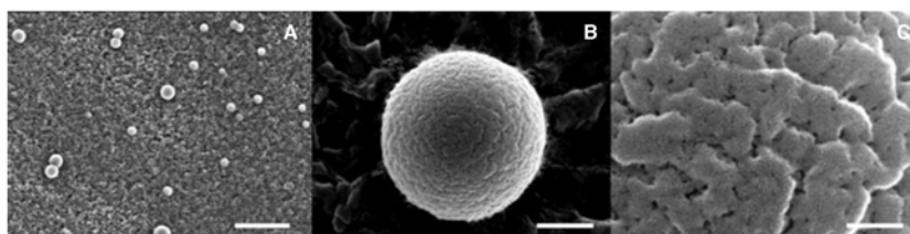
Fig. 6. Scanning electron micrographs of microspheres generated from LYS and apo \alpha -LA at different magnifications: (A) \times 2000 ; scale bar = 10 \mu\text{m} ; (B) \times 20\,000 ; scale bar = 1 \mu\text{m} ; (C) \times 100\,000 ; scale bar = 0.2 \mu\text{m} . Microspheres were obtained by mixing LYS (0.1 mM) with apo \alpha -LA (0.1 mM) in 30 mM Tris/HCl buffer, pH 7.5, containing 15 mM NaCl, and incubated for 30 min at 45 ^{\circ}\text{C} .
