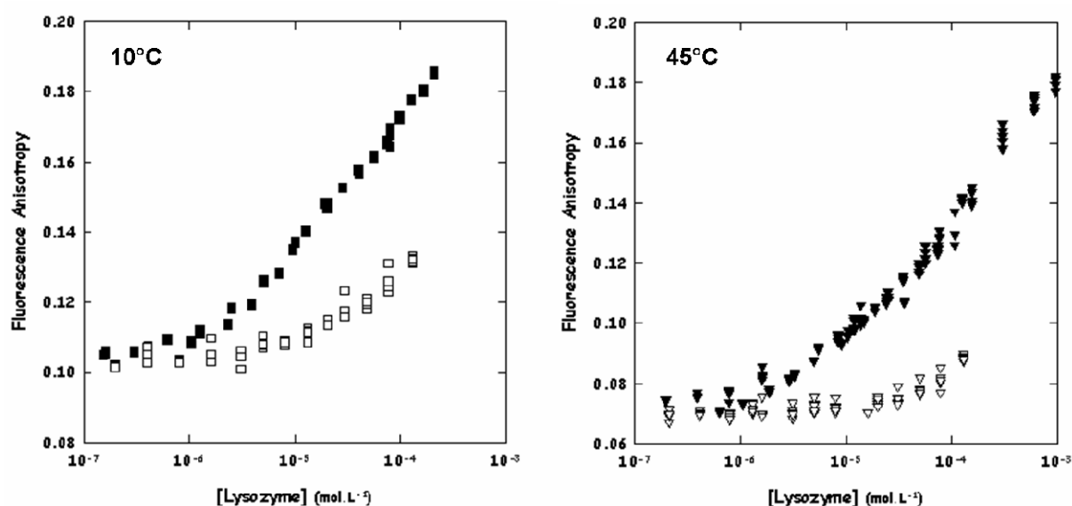
Figure 3. Holo \alpha -LA – LYS (closed symbols) and LYS – LYS (opened symbols) binding curves at 10^\circ\text{C} and 45^\circ\text{C} . [DNS labelled-protein] = 1 \times 10^{-6} \text{ mol.L}^{-1} . The ionic strength of the solution was 39 mM.
