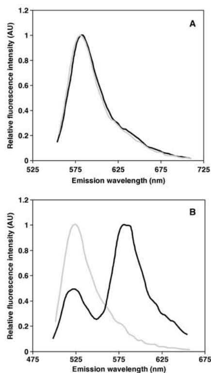
Fig. 5. Emission spectra of LYS-RBITC/apo \alpha -LA (gray) and LYS-RBITC/apo \alpha -LA-FITC (black) excited at 543 nm (A), and LYS/apo \alpha -LA-FITC (gray) and LYS-RBITC/apo \alpha -LA-FITC (black) excited at 488 nm (B).
