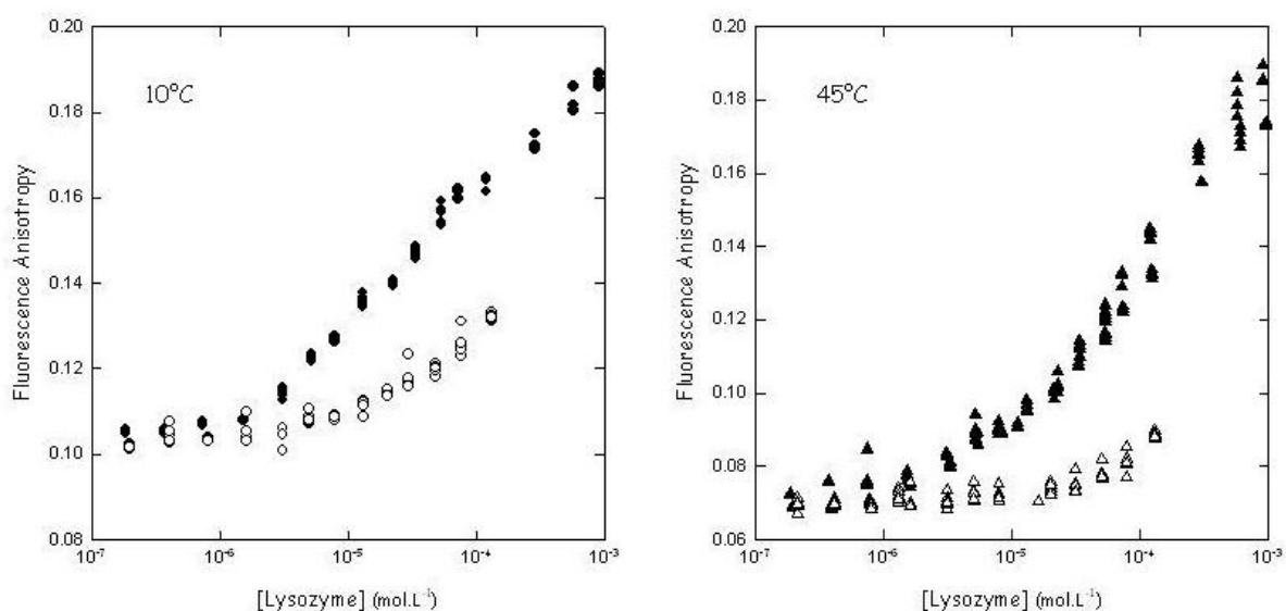
Figure 1. Apo \alpha -LA – LYS (closed symbols) and LYS – LYS (opened symbols) binding curves at 10^\circ\text{C} and 45^\circ\text{C} . [DNS labelled-protein]= 1 \times 10^{-6} mol.L ^{-1} . The ionic strength of the solution was 39 mM.
