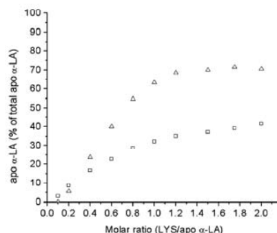
FIGURE 3: Proportion of apo \alpha -LA in the centrifuged material for different LYS/apo \alpha -LA molar ratios at 5 (□) and 45 °C (Δ). Mixtures of apo \alpha -LA and LYS were centrifuged at 12000g for 30 min at 5 or 45 °C. The pellets were washed with 30 mM Tris-HCl, 15 mM NaCl buffer (pH 7.5) and analyzed by rp-HPLC.
