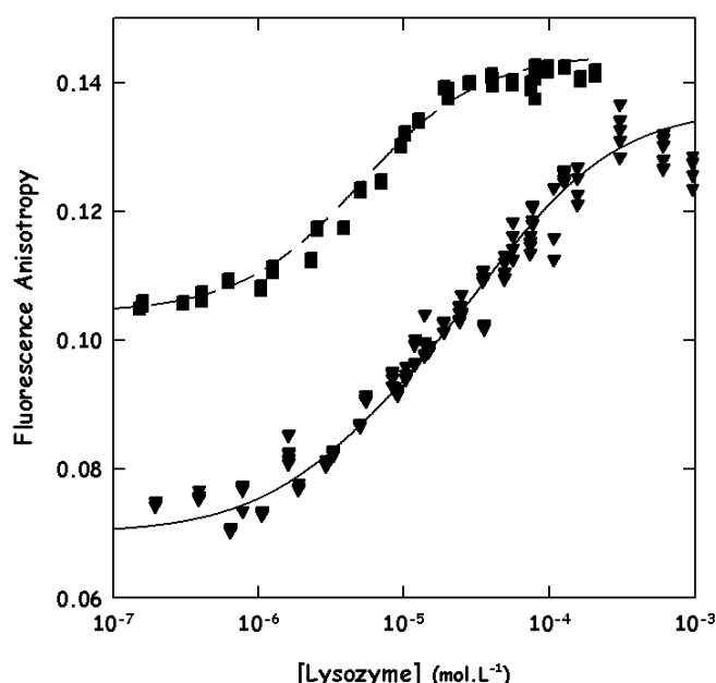
Figure 4. specific holo \alpha -LA – LYS binding curves at 10°C (■) and 45°C (▼). [\text{DNS-apo } \alpha\text{-LA}] = 1 \times 10^{-6} \text{ mol.L}^{-1} . The ionic strength was 39 mM.
