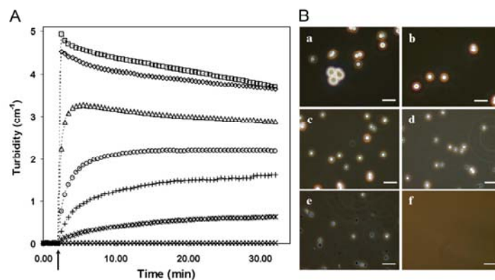
Fig. 1. (A) Kinetic formation of microparticles throughout mixing LYS (0.075 mM) and apo \alpha -LA (0.075 mM) in Tris/HCl buffers (5–30 mM), pH 7.5, with and without added NaCl (15–100 mM) at 45 °C. Final ionic strengths were: 4 mM (□), 24 mM (◇), 30 mM (△), 39 mM (○), 44 mM (+), 54 mM (κ) and 124 mM (×). The arrow shows the addition time of LYS to apo \alpha -LA. (B) Phase contrast micrographs of spherical particles taken 30 min after the mixture of LYS and apo \alpha -LA at different ionic strength (I): 4 mM (a), 24 mM (b), 39 mM (c), 44 mM (d), 54 mM (e) and 124 mM (f). The scale bar: 10 \mu m.
